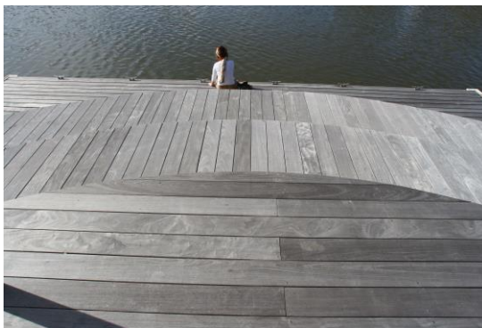
Top: Garapa unfinished / Bottom Left: Ipe finished with cedar tone penetrating oil / Bottom Middle: Ipe weathered / Bottom Right: Ipe finished with natural oil
